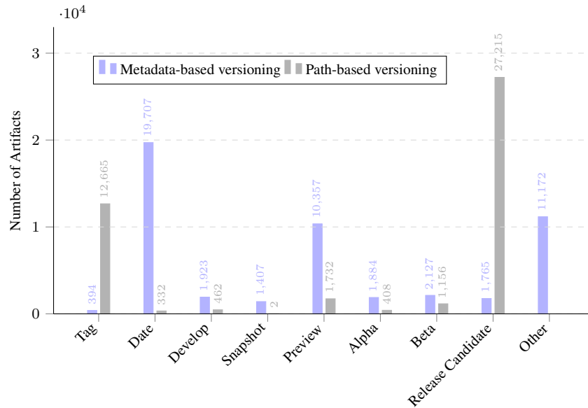
Figure 7: Comparing the adoption of the least used formats classed in metadata-based and path-based versioning in all datasets combined . (Semantic Versioning and Major Version Number have been omitted).
