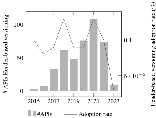
Figure 8: Header-based adoption in SwaggerHub Dataset over the year over the years
