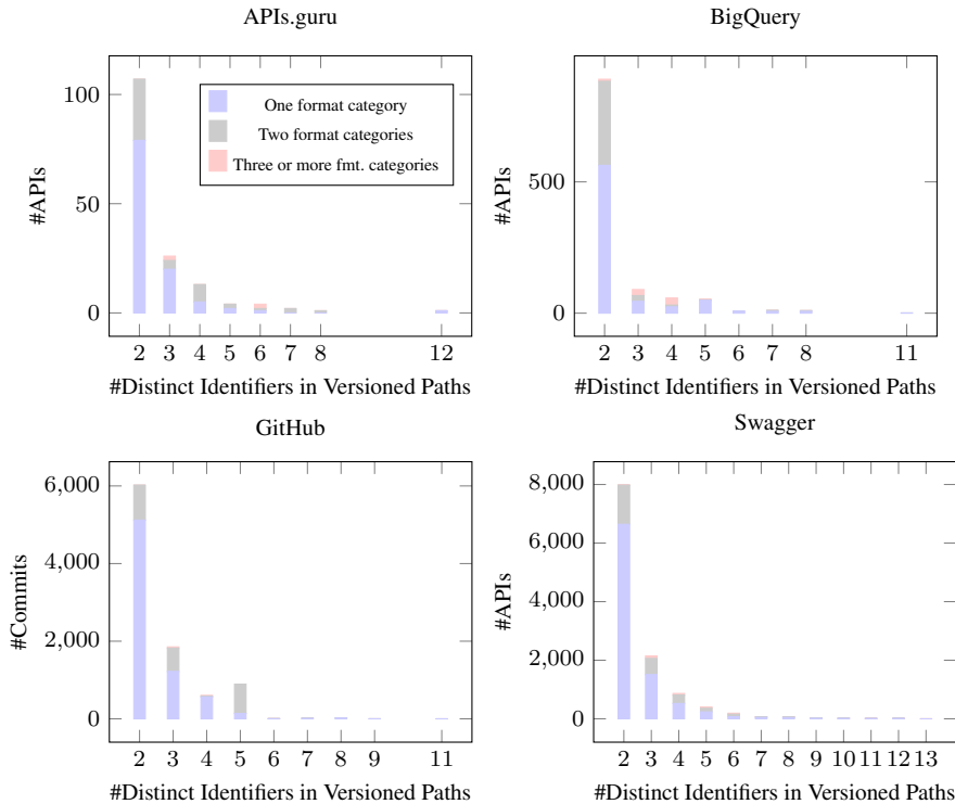
Figure 13: Usage of one or multiple format categories in path-based versioning of APIs with multiple versions in production
