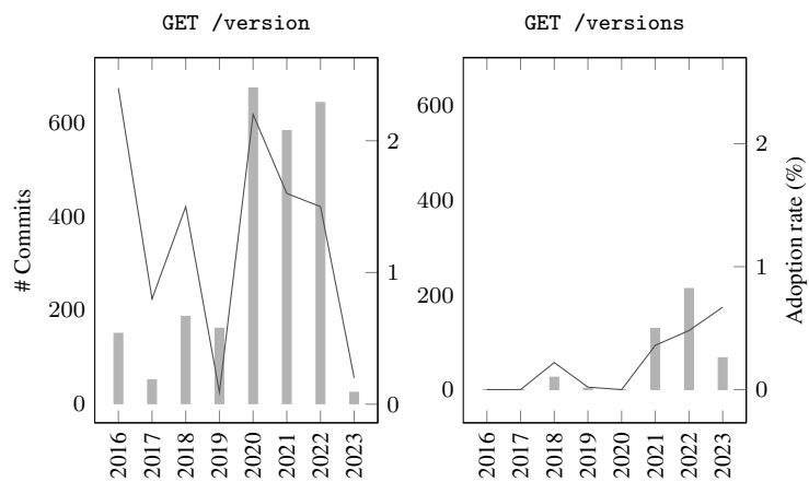
Figure 9: Dynamic versioning over the years in Github Dataset
